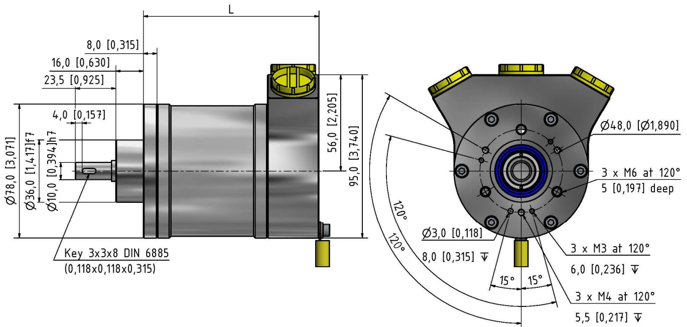
Face Mount C Clamping Flange
